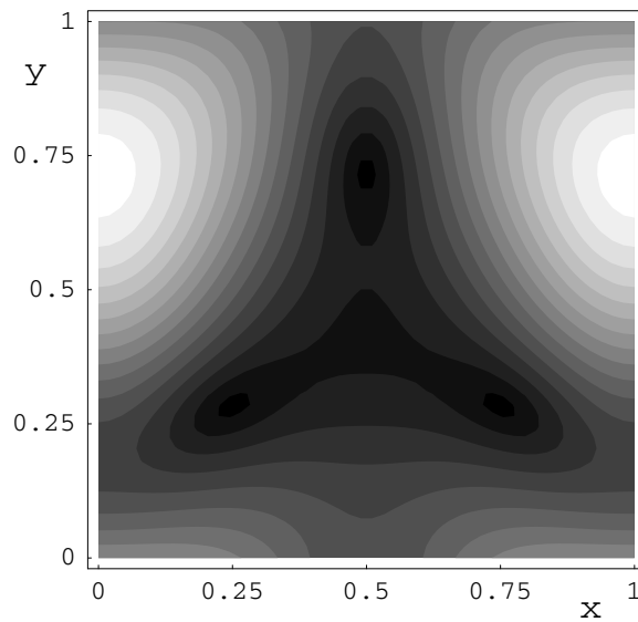
Figure 3. Modulo of the standard QPF whose phase plot is shown in figure 2. Darker regions correspond to lower values of the modulo. Because of the particular orientations of the major axes of the anisotropy ellipses, the modulo assumes its smallest values inside the triangle.
