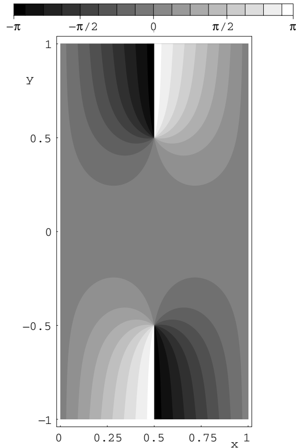
Figure 1. Phase of \vartheta_3[\pi(x+iy)|i] in two unit cells of quasiperiodicity, with one vortex per unit cell. The vortices, located at (x, y) = (0.5, \pm 0.5) , are positive and isotropic.
