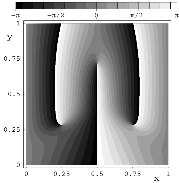
Figure 2. Phase of a standard QPF (27) with three vortices per unit cell. The vortices are located at the corners of an equilateral triangle (at the centre of the unit cell) with side length equal to 0.5. The two vortices at the basis of the triangle are positive while the third vortex is negative, giving a total vorticity N = 1 . All the vortices are anisotropic with eccentricity \varepsilon = \sqrt{3}/2 and the angles \theta between the major axis of the associated ellipse and the positive x axis are 30^\circ , 150^\circ and 270^\circ .
